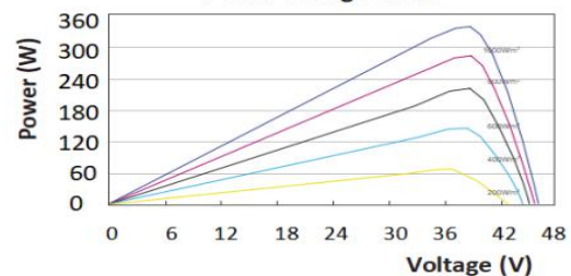
Power-Voltage Curve
